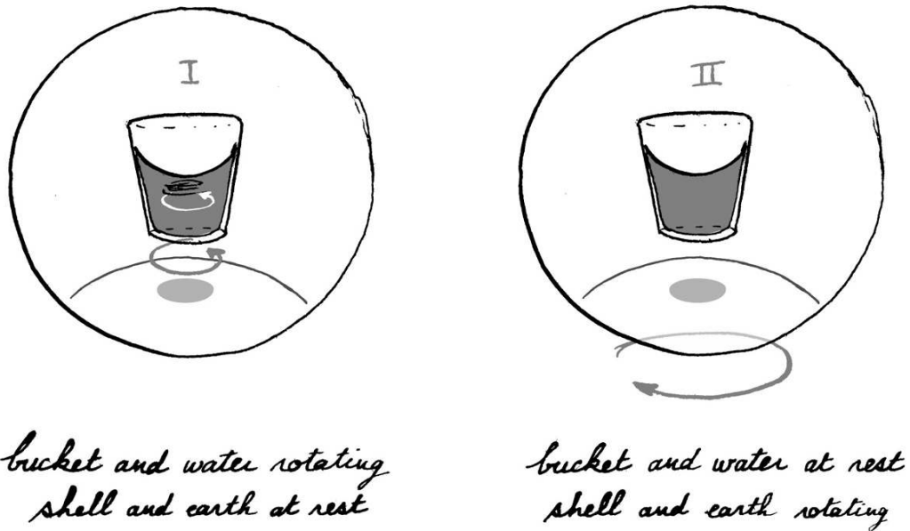
FIGURE 7. Machian account of Newton's rotating-bucket experiment.
