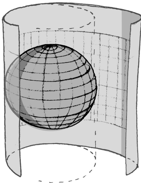
FIGURE 4. Mapping the earth.
