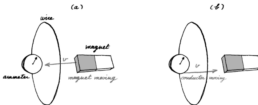
FIGURE 2. The magnet-conductor thought experiment.
