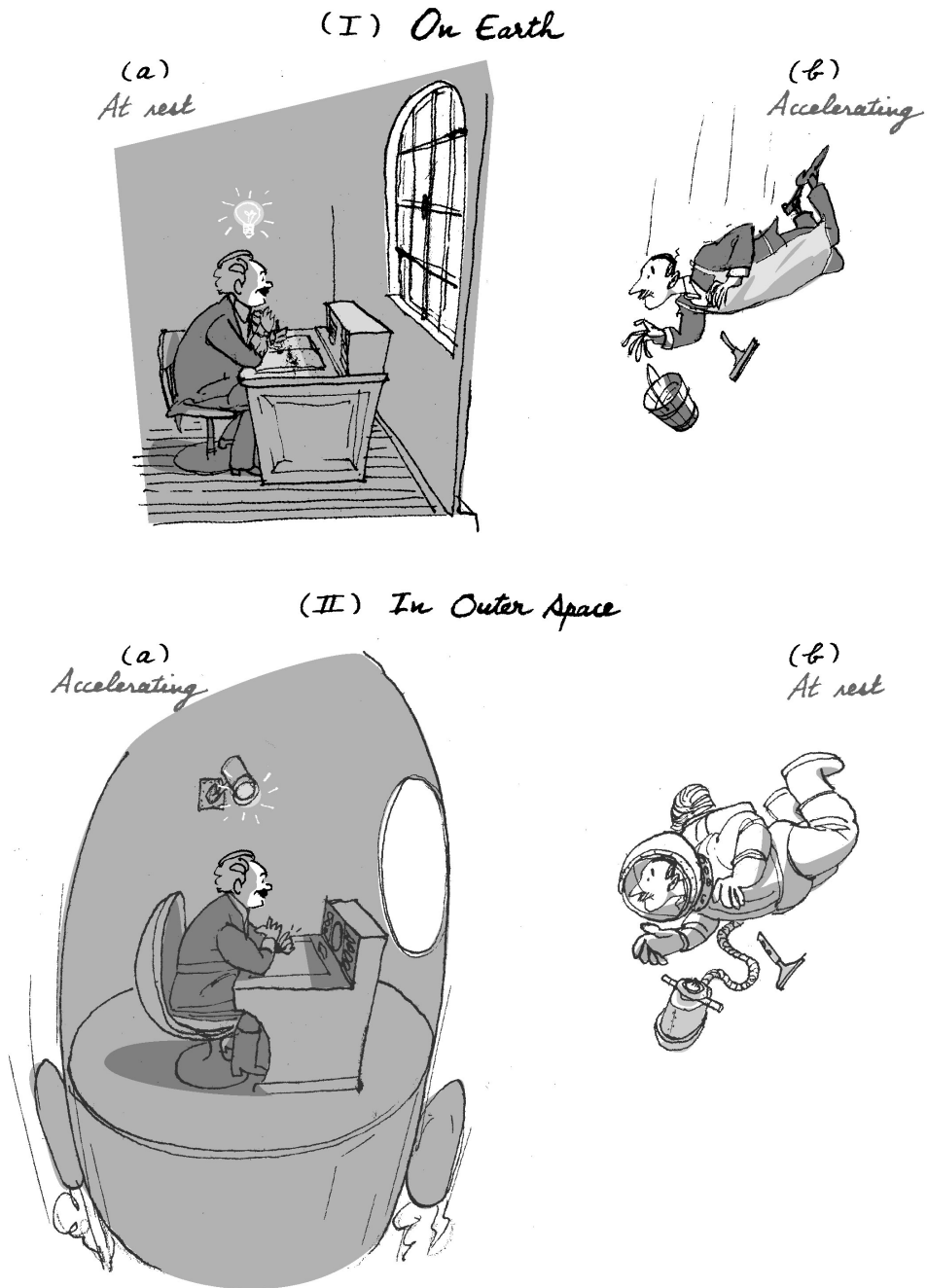
FIGURE 1. The equivalence principle. This and all other diagrams in this chapter were drawn by Laurent Taudin.
