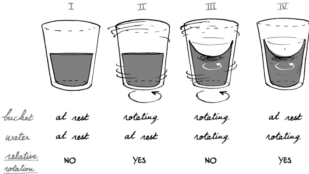
FIGURE 6. The rotating-bucket experiment.
