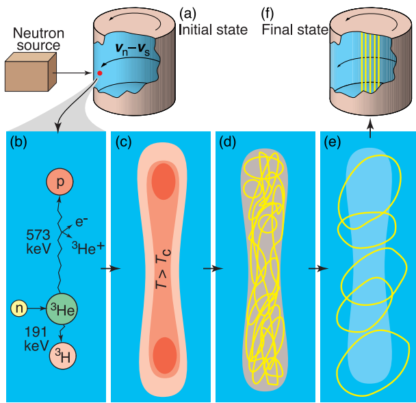
FIG. 10. Schematic illustration and interpretation of the Mini Bang experiment. See text for details. Figure modified from ref. 67.
