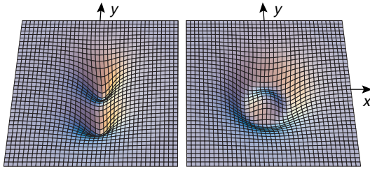
FIG. 5. Magnitude of the order parameter, \Sigma_i = 1,2,3 \Sigma_j = 1,2,3 |A_{ij}|^2 in the two types of vortex cores of ^3\text{He-B} : double-core vortex (Left) and A-phase-core vortex (Right). The magnitude is normalized to unity in bulk ^3\text{He-B} and has a minimum value of 0.5 in the two cores of the double-core vortex. The xy -plane is perpendicular to the axis of rotation. Vorticity is concentrated into regions where the order parameter is suppressed. The dimensions of the areas shown are on the order of 1 \mu\text{m} . Figure based on calculations in ref. 45.
