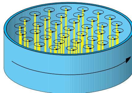
FIG. 1. Rotation of a superfluid is not uniform but takes place via a lattice of quantized vortices, whose cores (yellow) are parallel to the axis of rotation. Small arrows indicate the circulation of the superfluid velocity v_s around each singularity. The vortex array rotates rigidly with the container. The nearly hexagonal pattern of vortices applies to ^3\text{He-B} and ^4\text{He} .
