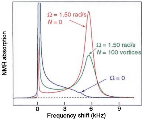
FIG. 4. NMR absorption spectra measured in rotating superfluid ^3\text{He-B} . See text for details. Figure reproduced with permission from ref. 44.
