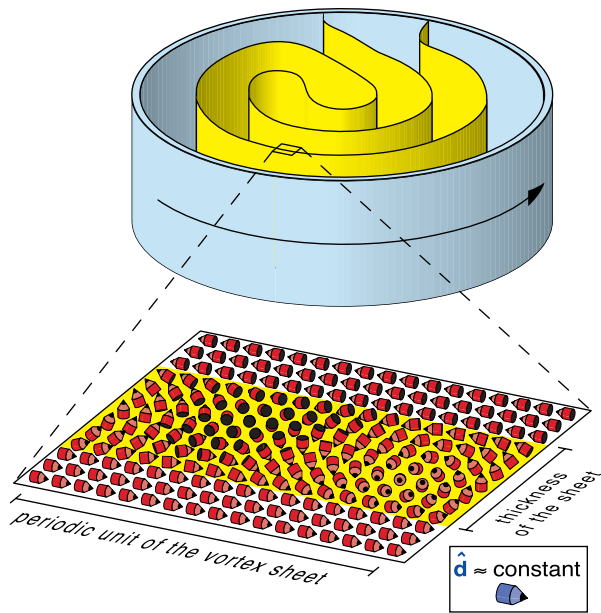
FIG. 9. Folding of the VS in a rotating container (Upper) and one periodic unit of the l -vector field associated with it (Lower). In the VS l is unlocked from d , which is pointing toward right, perpendicular to H . Figure adapted from ref. 55.
