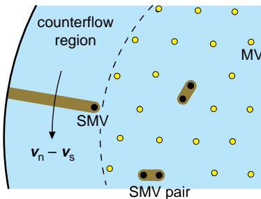
FIG. 6. SMVs in two different configurations. The yellow dots represent usual vortices that have only circulation of mass current (MV). The black dots are SMVs that are tied to a soliton tail (brown). Figure adapted from ref. 31.
