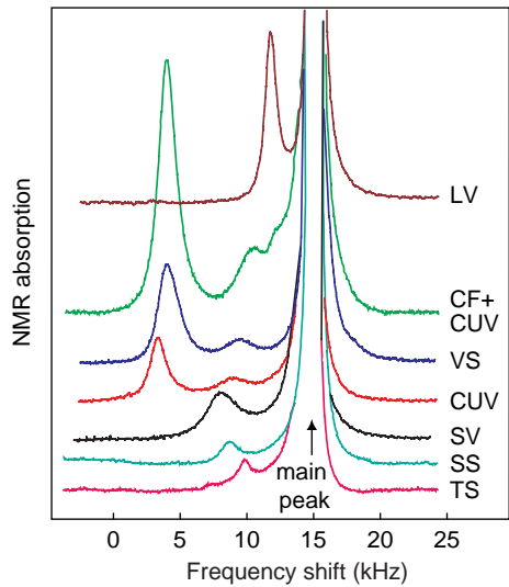
FIG. 8. NMR absorption spectra of different topological objects in rotating ^3\text{He-A} . In each case the main peak arises from the bulk liquid. Every defect (vortex or soliton) gives rise to a satellite peak at a characteristic frequency. The heights of the satellites are directly proportional to the number of each type of defect in the experimental cell. Compare with Fig. 7 and Table 1. For clarity the different spectra are shifted vertically. CF, counterflow region; SS, splay soliton; TS, twist soliton. Figure reproduced with permission from ref. 50.
