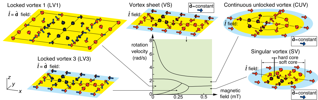
FIG. 7. Different types of l -textures in rotating superfluid ^3\text{He-A} . The phase diagram in the \Omega vs. H -plane is shown in the middle. The yellow shading denotes regions with vorticity, \nabla \times \mathbf{v}_s \neq 0 . In the blue areas outside, \text{curl } \mathbf{v}_s = 0 . Only half of the elementary cell is shown for VS and LV3. For more details, see text. Figure adapted from ref. 48.
