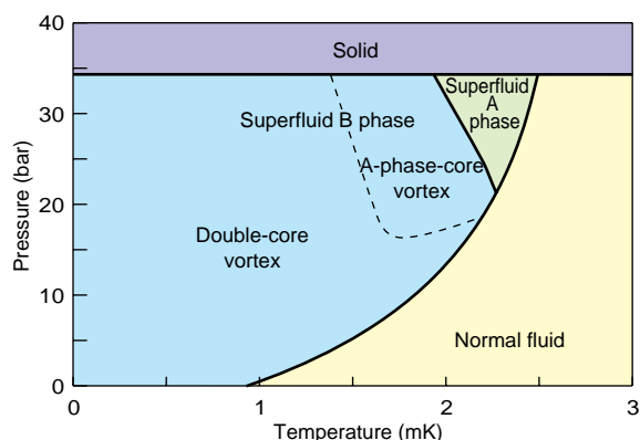
FIG. 2. Phase diagram of ^3\text{He} below 3 mK. The solid phase appears only above the pressure of 34 bar. At high temperatures the liquid is in the normal Fermi state. There are two superfluid phases, A and B. The transition line between the two types of vortex cores in rotating ^3\text{He-B} is shown by the dashed curve. Figure modified from ref. 5.
