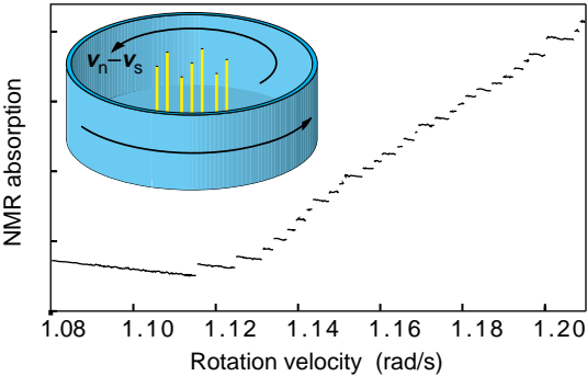
FIG. 3. NMR absorption near the Larmor frequency during acceleration showing the nucleation of single vortex lines, except the third last step that corresponds to two vortices. (Inset) A schematic illustration of a state with less than the equilibrium number of vortex lines. The singularities form a bundle in the center and are surrounded by a vortex-free counterflow region. Figure modified from ref. 44.
