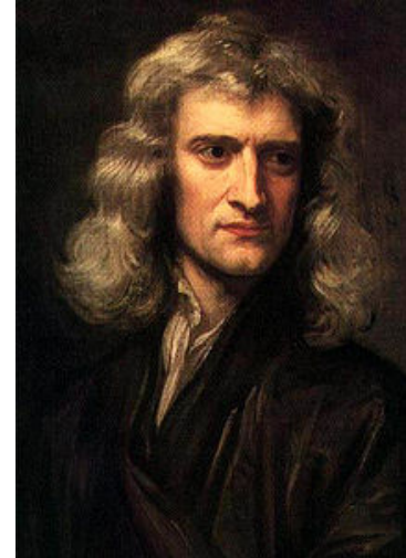
Theory of gravitation
