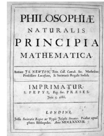
Theory of gravitation
