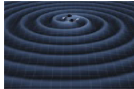
Ripples of warping in the fabric of space-time from orbiting black holes
