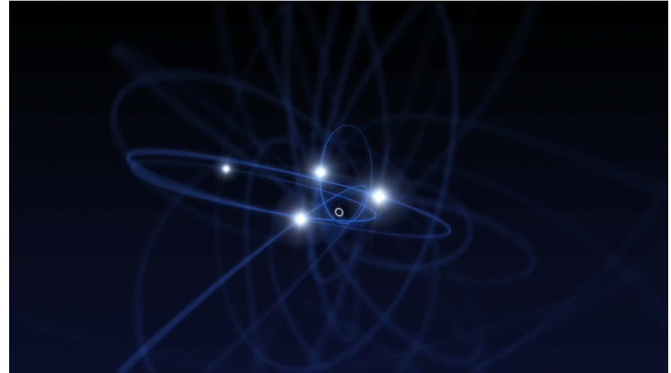
Black hole of 4 million solar masses in our galaxy's center
