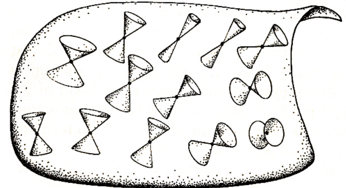
Elastic spacetime in general relativity
