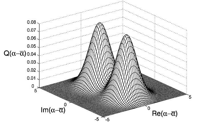
FIG. 2. The Q(\alpha-\bar{\alpha}) distribution calculated numerically from Eq. (2.19) in steady state. The bimodal structure of this distribution illustrates the two fixed points for the cavity field. These fixed points are separated along the phase quadrature by g/\kappa . Parameters used for this calculation are (g, \kappa, \Omega)/\gamma = (60, 20, 1200) . These parameters were chosen so as to show the clear separation of the fixed points.
