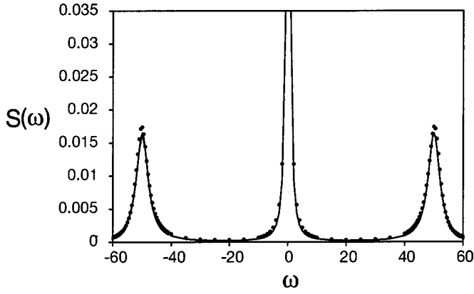
FIG. 11. Numerical (dots) and analytic (solid line) calculations for the fluorescence spectrum with no feedback. The parameters used are the same as in Fig. 9. Both axes are measured in units of \gamma .
