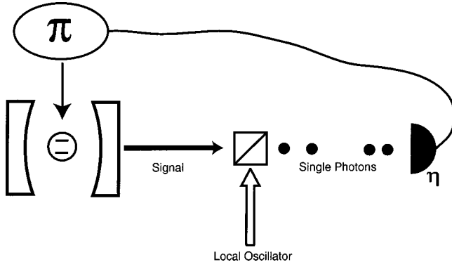
FIG. 5. The proposed direct detection scheme with a local oscillator to offset the large coherent field. The photodetector efficiency is given by \eta .
