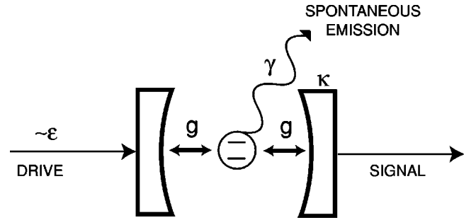
FIG. 1. An illustration of the single-atom cavity QED system.
