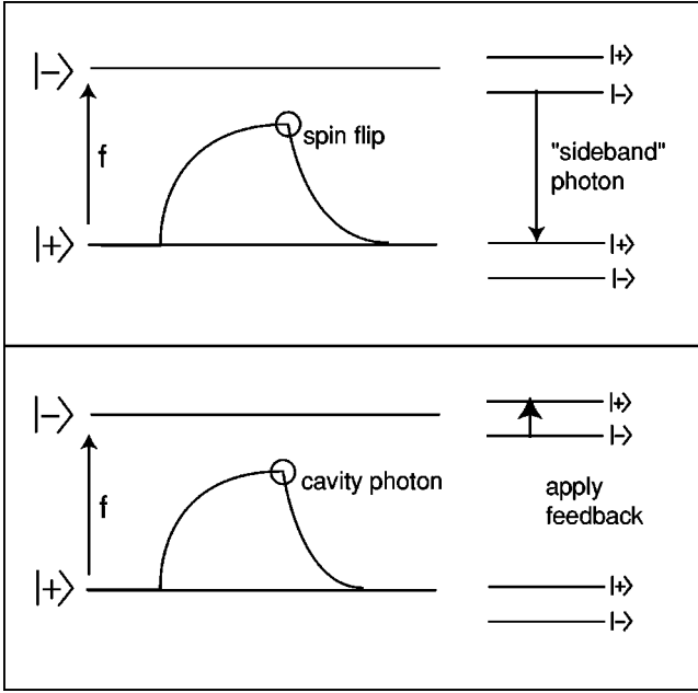
FIG. 8. Two possible events will keep the system in the |+\rangle dressed state. The top event goes undetected by the feedback loop, but leads to an unwanted sideband fluorescence photon. The bottom event is detected and suppresses the sideband photon.
