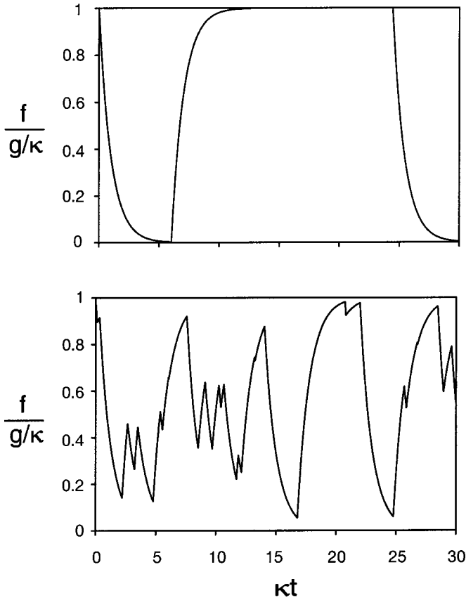
FIG. 6. Stochastic evolution of the cavity field following spontaneous-emission events. The top figure corresponds to \gamma/2\kappa = 2.5 while the bottom figure corresponds to \gamma/2\kappa = 0.067 , which are the same values used to calculate the distributions in Fig. 4. The parameter f = y/2 + g/2\kappa is the field displacement from the |+\rangle fixed point.
