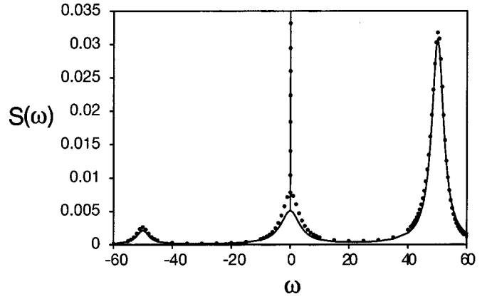
FIG. 12. Numerical (dots) and analytic (solid line) calculations for the fluorescence spectrum with feedback. Other details are as in Fig. 11.
