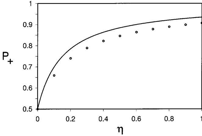
FIG. 9. Steady-state occupation of the |+\rangle state as a function of the detector efficiency. Numerical values are represented by dots and the approximate analytical expression is shown as a solid line throughout the rest of the paper. This plot was calculated with the following parameters: (\Omega, \kappa, g)/\gamma = (50, 15, 5) .
