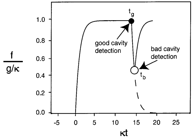
FIG. 7. Dynamics of the cavity field. A spontaneous emission flips the atomic state at t=0 . This is detected from the good detection at time t_g , and a feedback pulse is applied. If a bad detection subsequently occurs at time t_b then an unwanted second feedback pulse is applied, which puts the atom in the wrong state and drives the cavity field in the wrong direction. The dashed line shows where the field should go without the bad detection at t_b . As before the field is measured with the displaced operator f = (y + g/\kappa)/2 .
