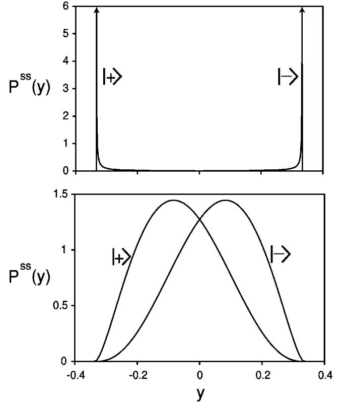
FIG. 4. Steady-state distributions of the cavity field for two different values of \gamma . The top graph corresponds to the semiclassical fixed point limit with \gamma/2\kappa=0.067 . The lower graph shows the mixing of the field states when \gamma/2\kappa=2.5 . g/\kappa=0.33 for both plots.
