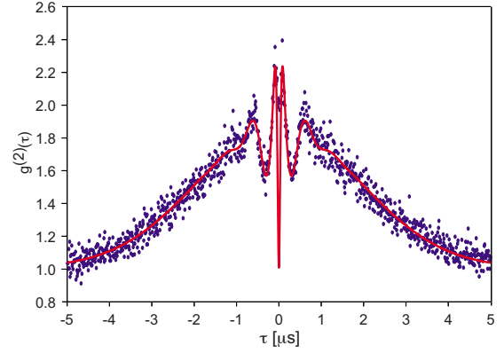
FIG. 8. (Color online) Intensity autocorrelation function [g^{(2)}(\tau)] of the perpendicular mode at 0.24n_0 . The continuous line is the theoretical fit to Eq. (12).
