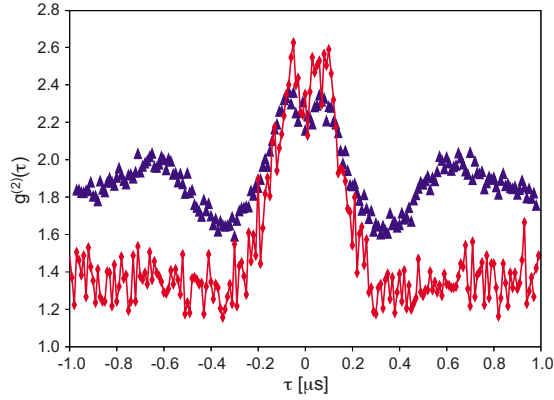
FIG. 7. (Color online) Intensity autocorrelation function [g^{(2)}(\tau)] of the perpendicular mode with (triangles) and without (diamonds) Faraday rotation at a driving intensity of 0.4n_0 .
