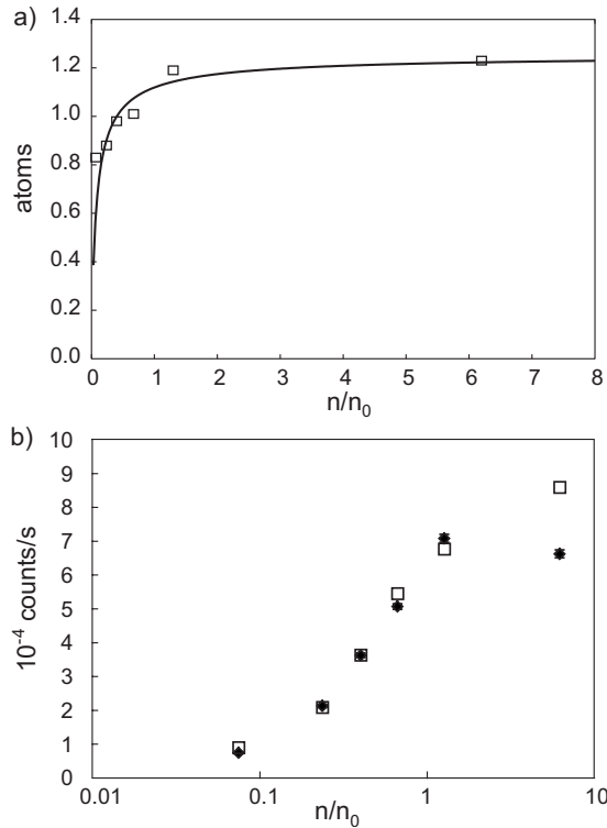
FIG. 10. (a) Measured mean number of interacting atoms and theory curve showing the expected saturation. (b) Measured (filled rhombs) count rates in the perpendicular mode together with those predicted from the extracted mean number of atoms (open squares), photons per atom, and transit time.
