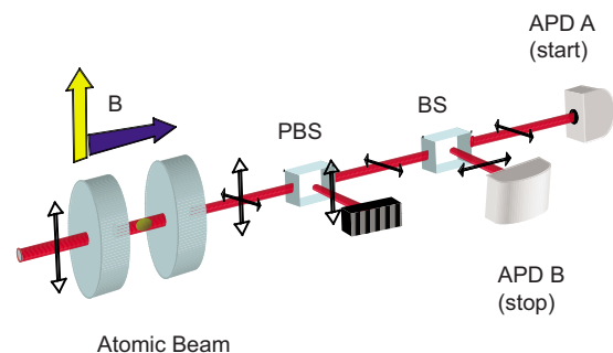
FIG. 1. (Color online) Schematic of the apparatus with the basic optical elements necessary for coincidence measurements. Vertically polarized laser light (parallel) drives the high finesse cavity traversed by a continuous beam of cold ^{85}\text{Rb} atoms from a magneto-optical trap. The output light passes through a polarizing beam splitter (PBS) that separates the horizontal (perpendicular) polarization, sending it to a nonpolarizing beam splitter (BS) for coincidence measurements using two avalanche photodiodes (APDs). The direction of the magnetic field (B) inside the cavity can be parallel to the polarization ( \pi -polarized drive) or parallel to the direction of propagation ( \sigma -polarized drive).
