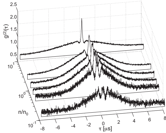
FIG. 9. Intensity autocorrelation function [g^{(2)}(\tau)] of the perpendicular mode for different values of photon number (intensity) in the driven mode.
