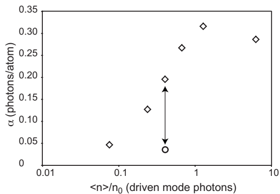
FIG. 5. Counts detected from a single atom (rhombus for Faraday; circle for non Faraday) as a function of intensity of the exciting laser normalized by the saturation photon number. The arrows indicate the points extracted from the plots on Fig. 4. The error bars are smaller than the size of the data points.
