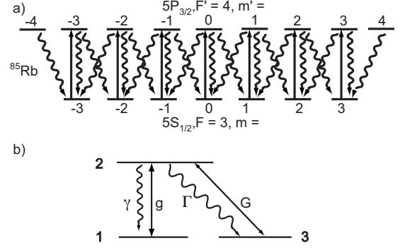
FIG. 3. (a) Diagram of ^{85}\text{Rb} levels relevant to the detection. (b) Energy level diagram of the simplified model.
