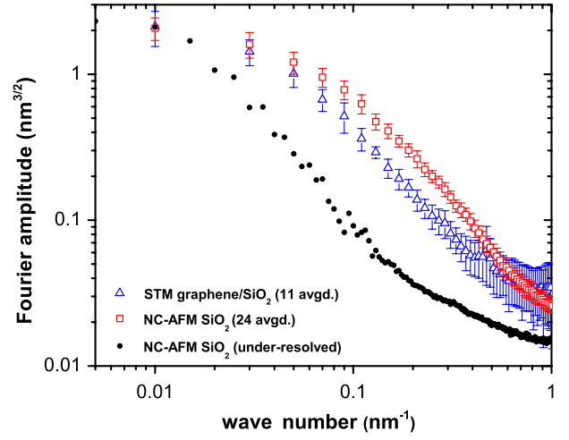
FIG. 2 (color online). Fourier amplitude spectra of: SiO 2 NC-AFM (red squares), monolayer graphene/SiO 2 STM (blue triangles), and under-resolved SiO 2 (black dots). Spectra 1 and 2 were obtained from an averaged data set to establish statistical uncertainty, as discussed in the supporting information. Wave number is defined as wavelength −1 .
