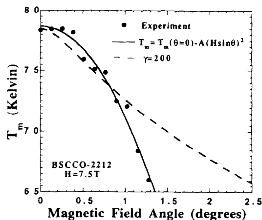
Figure 2. T - \theta diagram for BSCCO-2212 with H=7.5 Tesla \parallel ab -plane.
