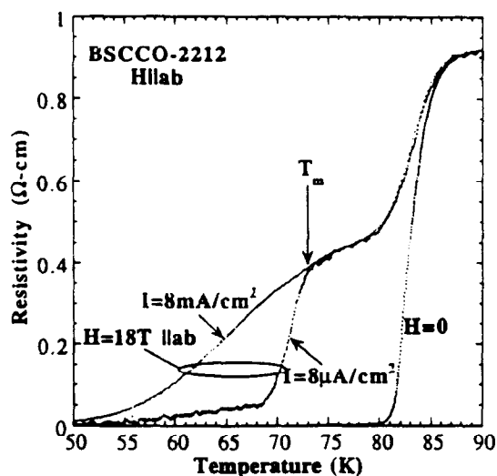
Figure 1. The c-axis resistivity of BSCCO-2212 at 18 Tesla \parallel ab for two different measuring current densities. The zero field data are also shown.
