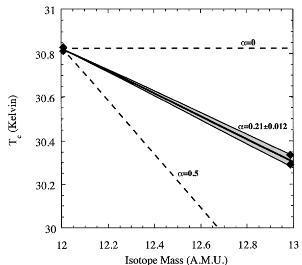
FIG. 2. The superconducting transition temperature, T_c , of two samples each of Rb_3^{12}C_{60} and Rb_3^{13}C_{60} versus isotopic mass. The solid line fits T_c \propto M^{-\alpha} , and gives \alpha = 0.21 \pm 0.012 . Dotted lines show \alpha_C = 0 and \alpha_C = 0.5 for comparison. The shaded area represents the error bars for this measurement.
