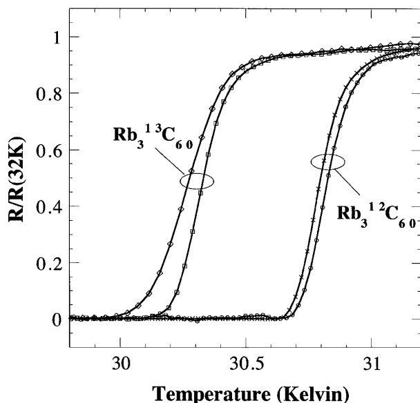
FIG. 1. The resistance (normalized to its value at 32 K) of two samples each of Rb_3^{12}C_{60} and Rb_3^{13}C_{60} versus temperature. Solid lines guide the eye.
