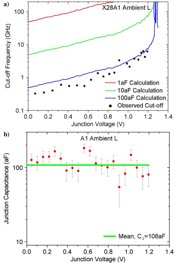
Fig. 6. (a) Calculated bias-dependent cutoff frequency f_c(V) assuming various trial junction capacitance values [ 1 \text{ aF} (in red in online version), 10 \text{ aF} (in green in online version), 100 \text{ aF} (in blue in online version)] and the observed cutoff frequencies (black circles) for a 20\text{-}\mu\text{m} -long device. (b) Experimentally determined junction capacitance as a function of frequency (red circles in online version), extracted from the observed cutoff frequency using (5). Green line (in online version) shows the mean value of the junction capacitance of 108 \text{ aF} .
