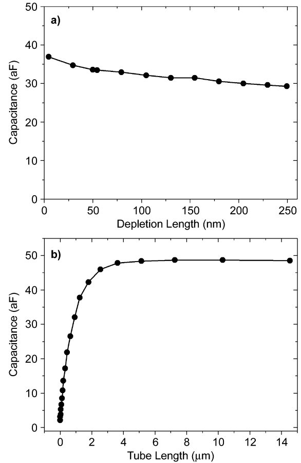
Fig. 10. Results of capacitance calculated from 3-D numerical simulations, showing a much stronger dependence on channel length than depletion length.
