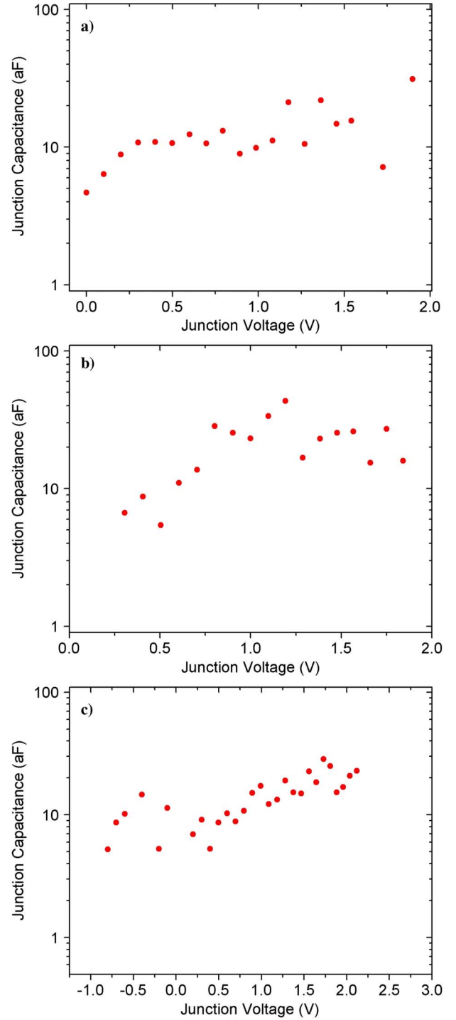
Fig. 8. Extracted junction capacitance in vacuum as a function of dc bias for CNT-SDs with channel lengths of: (a) 1 \mu\text{m} , (b) 3 \mu\text{m} , and (c) 7 \mu\text{m} .
