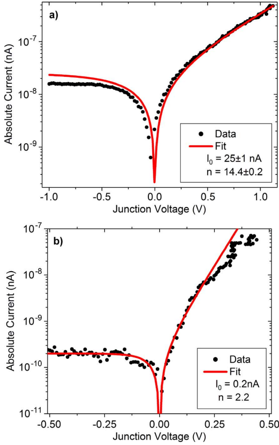
Fig. 3. Measured I - V characteristics of two CNT-SDs (black dots) with superimposed fits (red solid lines in online version) to the Shockley diode equation (1).
