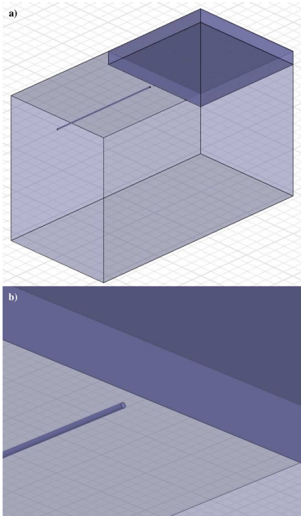
Fig. 9. 3-D model used for numerical capacitance calculations. (a) Overall view of the conducting cylinder and rectangular electrode on a quartz substrate and (b) close-up view of the gap between the channel and electrode, which represents the depletion region.
