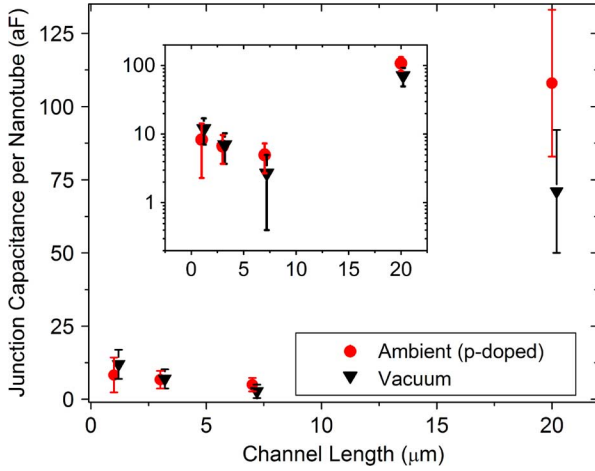
Fig. 7. Capacitance per nanotube channel as a function of device length; data are also in Table I. The vacuum values are slightly offset for clarity. Inset: Log-linear scale.
