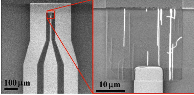
Fig. 1. (left) SEM image of the CPW electrode geometry and (right) close-up of the active device area. The center electrode (bottom feature on the close-up) is the Schottky contact, while the outer electrode (top in the close-up) is ohmic.
