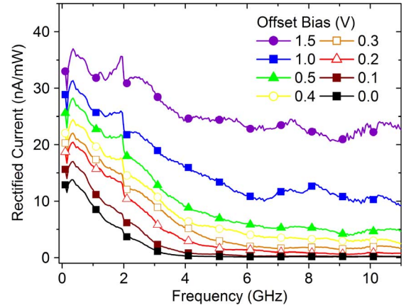
Fig. 5. Rectified current (in units of nanoamps per milliwatt) for a CNT-SD as a function of ac frequency and dc offset bias.
