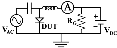
Fig. 4. Circuit diagram for the measurement setup showing the diode (DUT) connected to a bias tee (capacitor and inductor), microwave source ( V_{AC} ), dc source ( V_{DC} ), and a lock-in amplifier.
