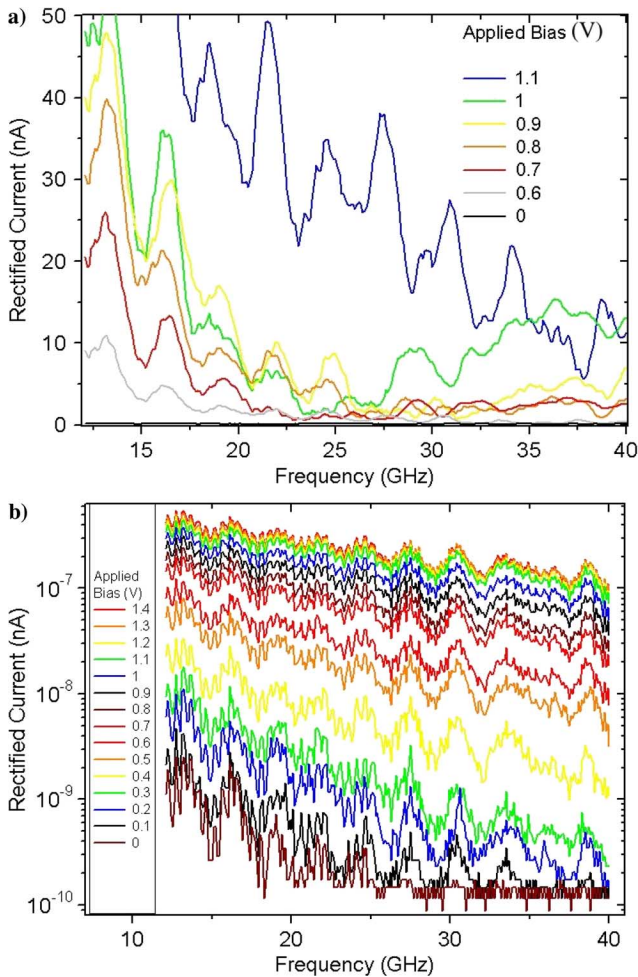
Fig. 12. Rectified current signal from a CNT-SD showing: (a) bias-dependent minima in the rectified signal at 26 GHz and (b) bias-dependent SNR of 500 at 40 GHz.
