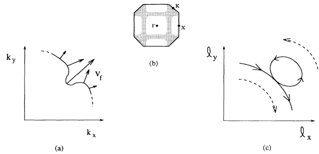
FIG. 4. (a) Blowup of the disordered Fermi surface, showing variation in v_f near a region of negative curvature (a "dip"). The Fermi velocity is larger toward the origin which is the center of a large electronlike region. (b) Large-scale view of Fermi surface. Shading delineates region containing the complex disordered Fermi surface. Adapted from [4]. (c) Circuit traced by scattering length vector \vec{l} = \tau\vec{v}_f corresponding to the portion of Fermi surface shown in (a). The circulation in the secondary loop is opposite to that in the primary loop. A similar argument applies to "bumps" in the Fermi surface.
