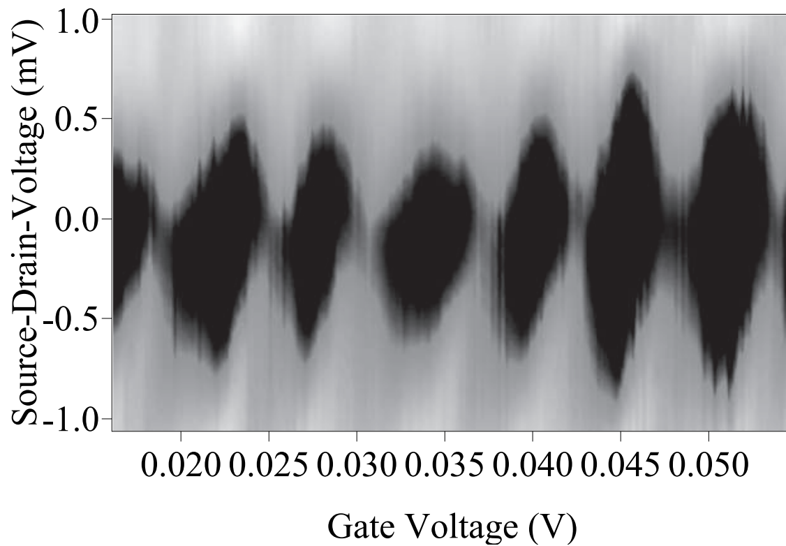
Figure 3.4: Coulomb Oscillations in a nanotube-SET measured at a temperature of 470 mK. The image shows the device conductance as it changes with V_{sd} and V_g . Darker tones indicate lower conductance. (The detailed conductance scale is shown with figure 5.5.)
