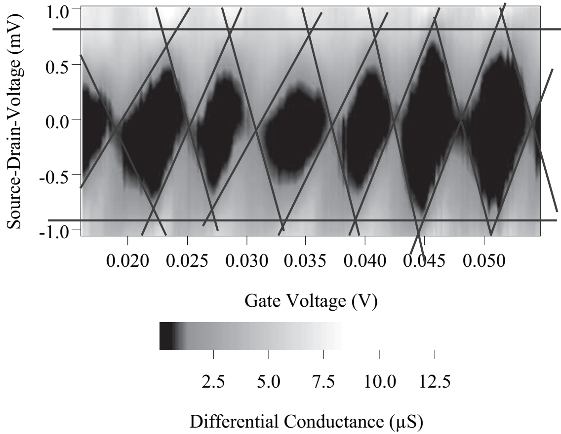
Figure 5.5: Differential conductance as a function of both V_{sd} and V_g of device EF measured at 470 mK. The lines indicate how the charging energy E_C was extracted from this plot.
