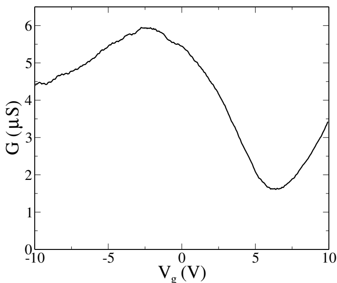
Figure 4.6: Conductance as a function of applied gate voltage for a typical device fabricated from a nanotube fabricated with the technique for thin tubes measured with a bias voltage of V_{sd} = 10 mV. Clearly the device does not turn off for any gate voltage as expected from a semiconducting nanotube. Unlike for metallic nanotubes, however, the conductance modulates strongly with V_g .
