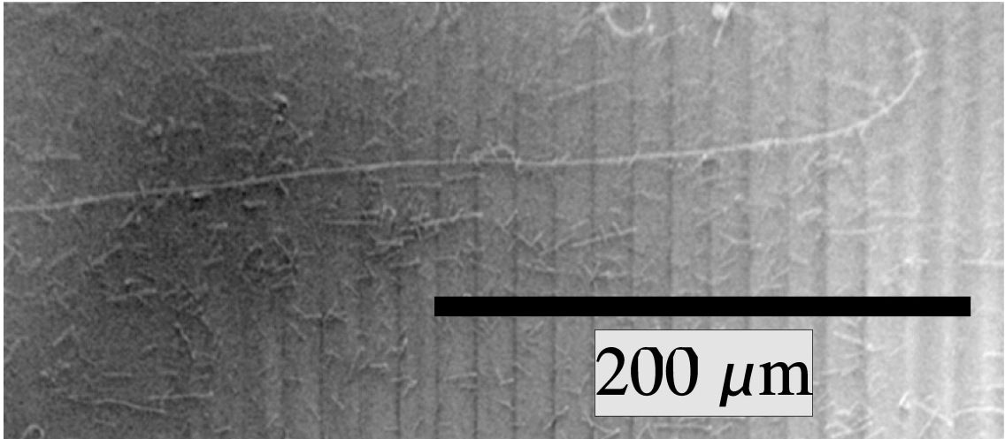
Figure 4.4: Scanning electron microscope (SEM) image of nanotubes grown with the \text{H}_2/\text{CH}_4/\text{C}_2\text{H}_4 gas mixture. One long nanotube is shown in front of a background of short tubes.
