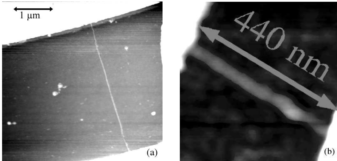
Figure 5.1: AFM micrographs of nanotube SETs. The contacts were fabricated with the technique described in section 4.2 on page 43 using a Cr adhesion layer and Au; the nanotubes themselves were grown with the “doughnut” method (section 4.1.1). (a) Tube EF. The distance between the contacts along the nanotube is 3.5 \mu\text{m} . (b) Tube FG. The device length is 440 nm.
