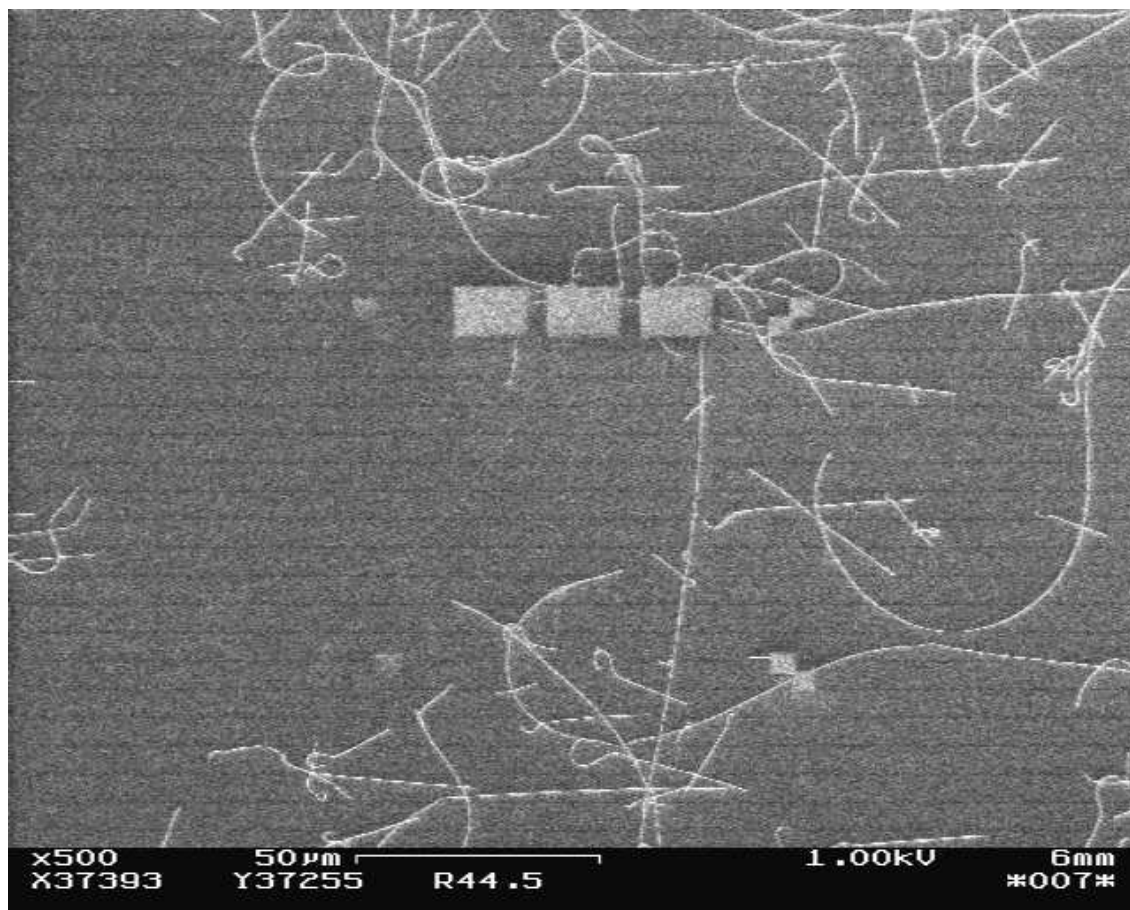
Figure 4.2: Scanning electron microscope (SEM) image of nanotubes grown with the “doughnut” method. On this particular sample the nanotube density is too high for device fabrication. The square and rectangular shaped objects are part of the alignment mark pattern explained in section 4.2.
