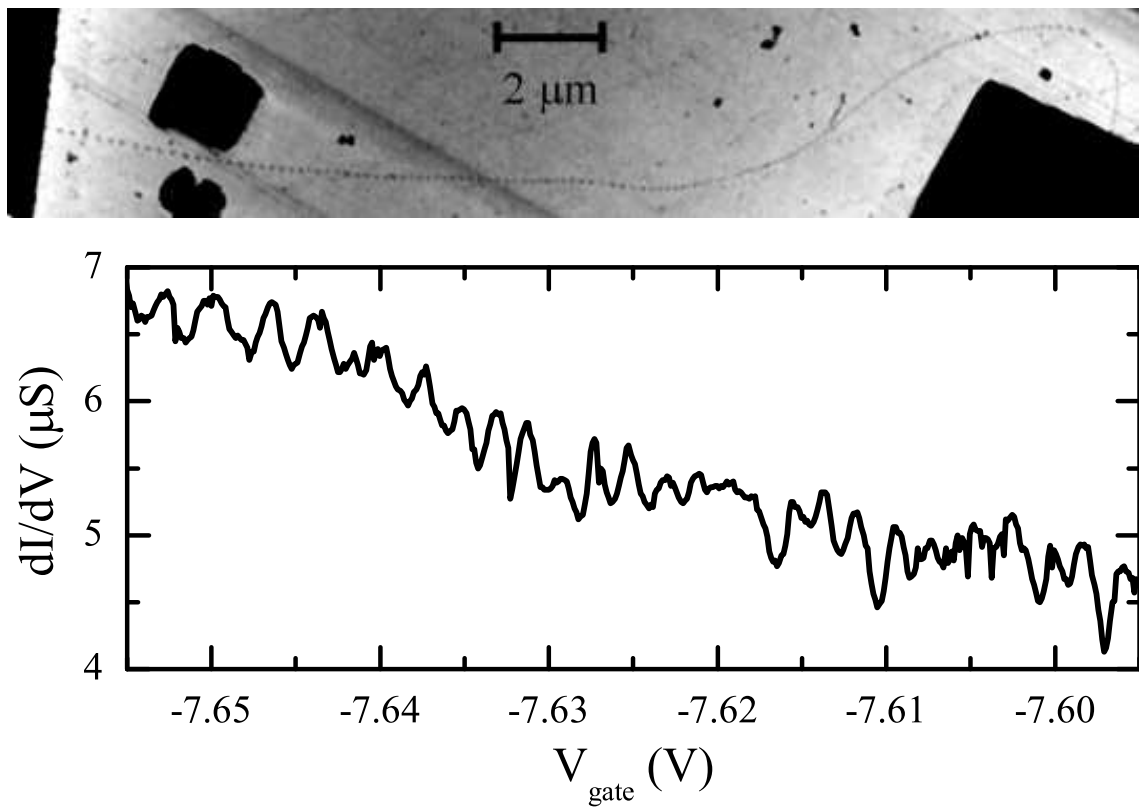
Figure 5.7: AFM micrograph of a 20 \mu\text{m} long semiconducting nanotube (device BF, sample 58 with a diameter d = 2.2 nm) and Coulomb oscillations measured on this device at a temperature of 470 mK using the AC-technique described in section 4.3. The DC-component of V_{sd} was set to zero in this measurement.
