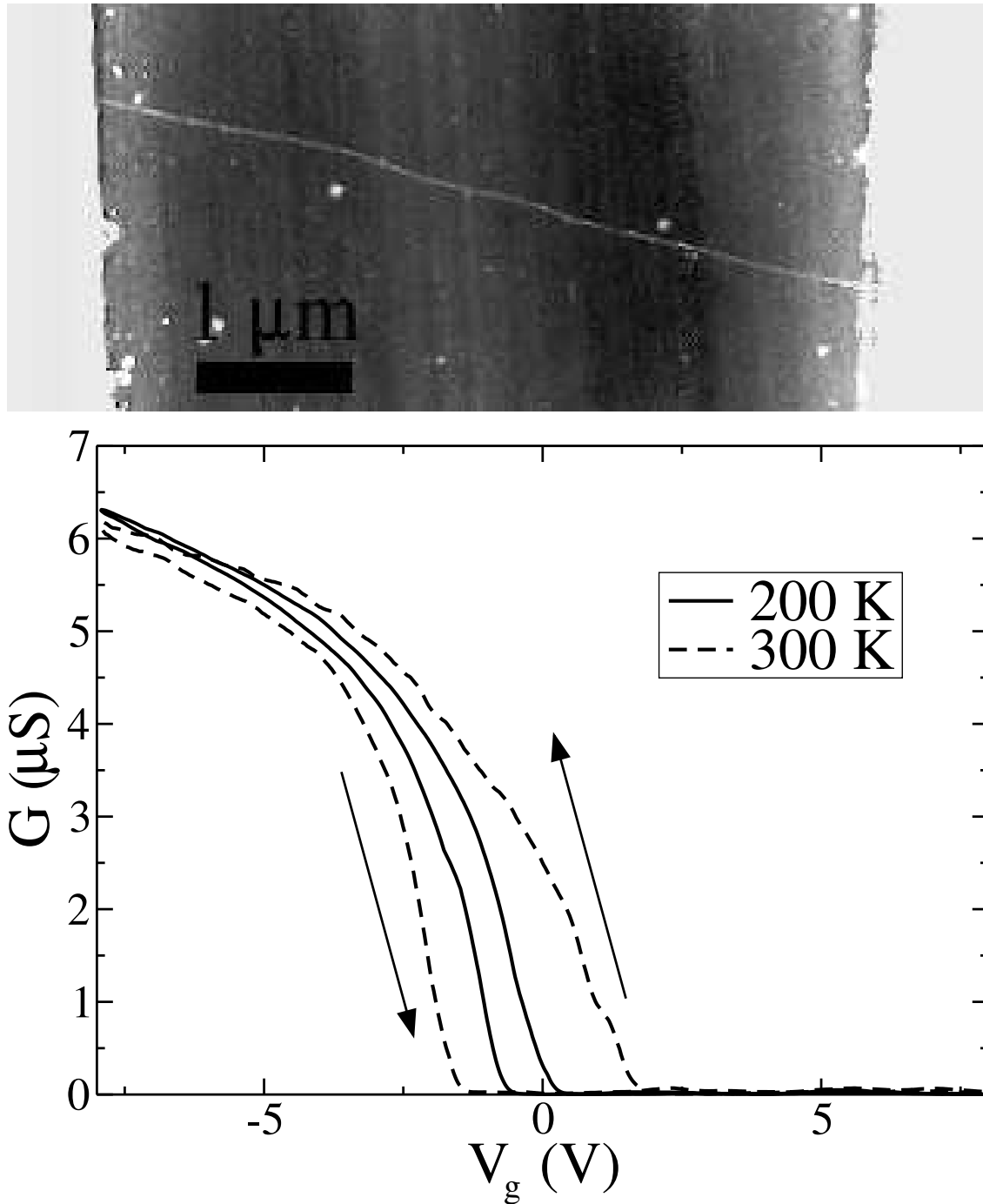
Figure 7.1: 4.8 \mu\text{m} long semiconducting nanotube with a diameter of 2.7 nm, device AB on sample 58: AFM-micrograph of the device and hysteresis loops in the G(V_g) -curve of the device at 200 K and 300 K. The data was measured with a bias voltage of 500 mV. The arrows indicate the direction in which V_g was being swept on each branch of the hysteresis. (Measurement courtesy of M. Fuhrer.)
