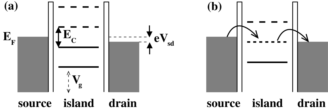
Figure 3.6: Quantum mechanical description of an SET: (a) The states in the metallic source and drain contacts are filled up to the Fermi energy. For the island the energy levels for (N - 1) , N , (N + 1) and (N + 2) electrons are shown. An applied V_g shifts these levels relative to the contacts. In this situation none of the states is within the energy interval given by V_{sd} making it impossible for electrons to tunnel onto or off the island. The device does not conduct. (b) By applying a suitable V_g a state on the island is pushed between the Fermi levels of source and drain allowing tunneling. The SET conducts.
