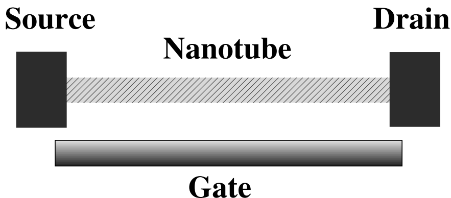
Figure 3.1: Schematic of a nanotube transistor. The nanotube acts as a channel between source and drain contacts. The gate is used to control the resistance of the channel. By applying a voltage to the gate it is possible to control the resistance of the device.
