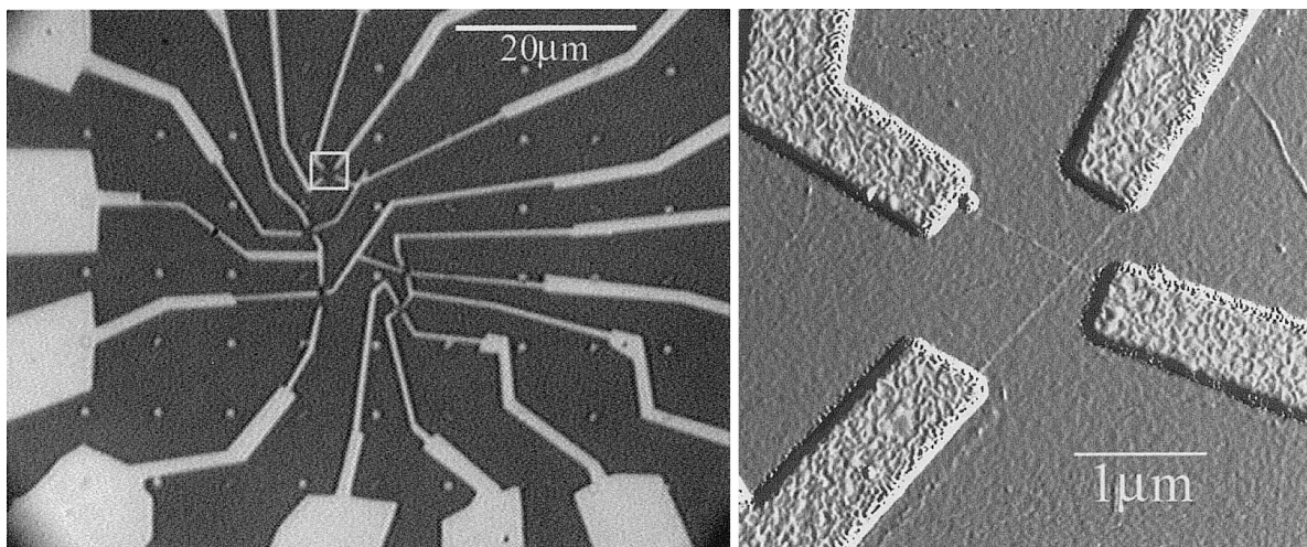
Fig. 1. (a) Optical micrograph showing Cr/Au electrical leads to five crossed SWNT devices. (b) Tapping mode AFM image (amplitude signal) of the area indicated by the white box in (a). Two SWNT are evident spanning between the Cr/Au electrodes.
