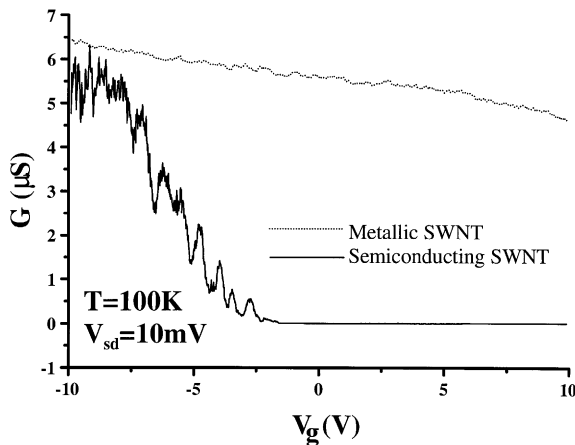
Fig. 2. Two-terminal conductances of individual metallic and semiconducting nanotubes as a function of gate voltage.
