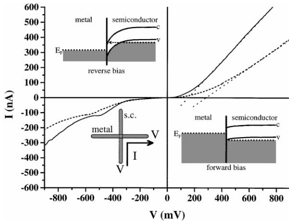
Fig. 4. Current as a function of bias voltage (applied to the semiconducting SWNT) for two metal–semiconductor SWNT junctions. The dotted lines are linear fits to the forward bias data (see text).
