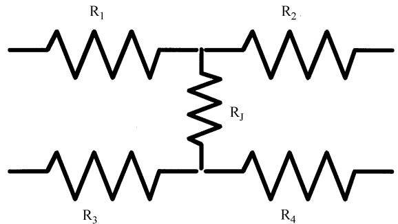
Fig. 3. Resistor network model for crossed SWNT devices.
