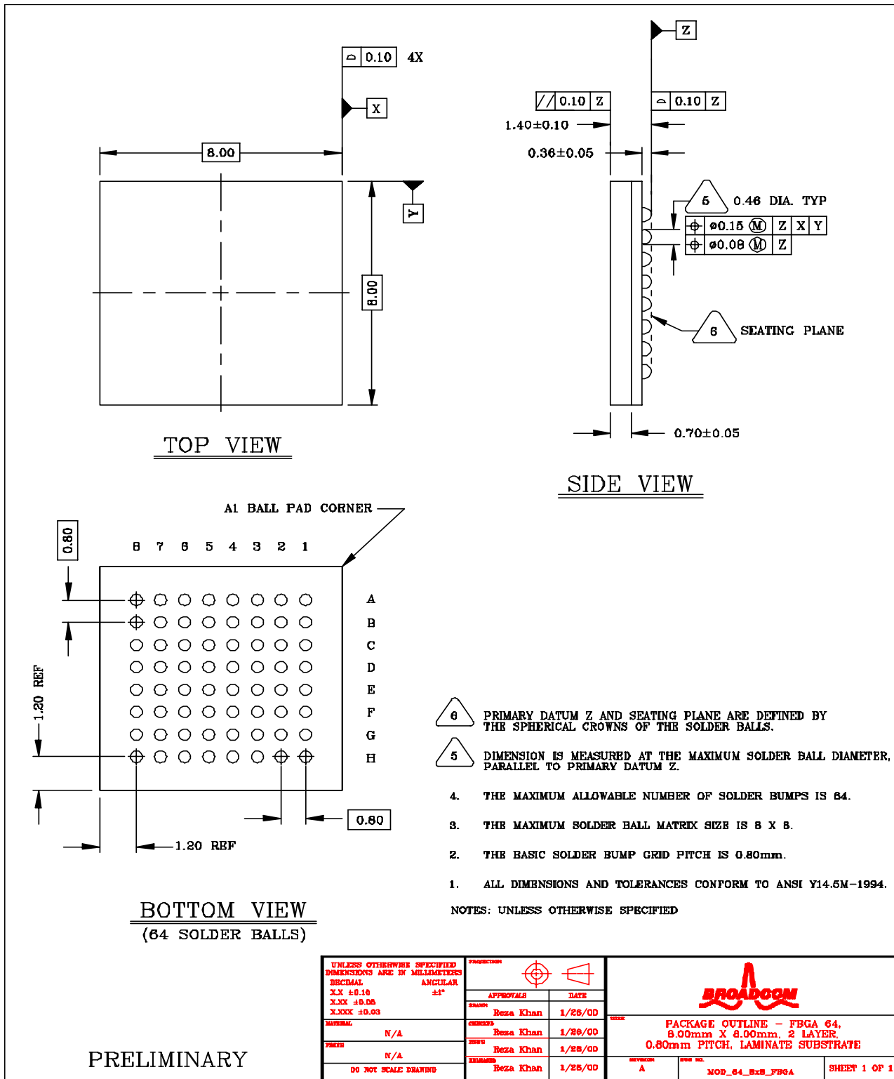
Figure 20: FBGA 64, 8mmx8mm (BCM5221 KP)
