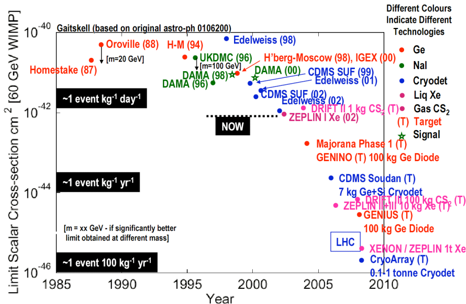
Figure 1. Experimental sensitivities (90% upper CL) for 60 GeV WIMP-nucleon scalar cross-section ( 10^{-46} \text{cm}^2 is equivalent to 10^{-10} \text{pb} ) versus times of publications. (Not meant to be an exhaustive selection.) The labels in the boxes give the equivalent event rates in Ge assuming a low recoil energy threshold >10 \text{keV} . Also shown are a selection of the maximum sensitivities for a number of planned experiments. The standard vanilla assumptions are made about the WIMP population in the Galaxy (Lewin&Smith): local density of 0.3 \text{GeVcm}^{-3} , and a characteristic velocity of 230 \text{kms}^{-1} . The SUSY physics reach of the 1 tonne experiments will be broadly comparable to that of the LHC which is due to report results before the end of this decade.
