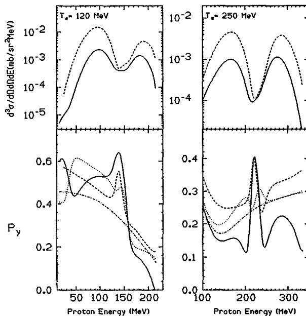
FIG. 3. Calculations of ^{12}\text{C}(\pi^+, 2p)^{10}\text{B}(3^+; 0.0 \text{ MeV}) . Outgoing proton angles are the same as in Fig. 1. PWIA results are shown as dash lines, free \pi^+ + {}^2\text{H} \rightarrow 2p polarizations are shown as dash-dot lines, dotted lines are no-spin-orbit DWIA polarizations, and finally continuous lines represent DWIA results including spin-orbit terms.
