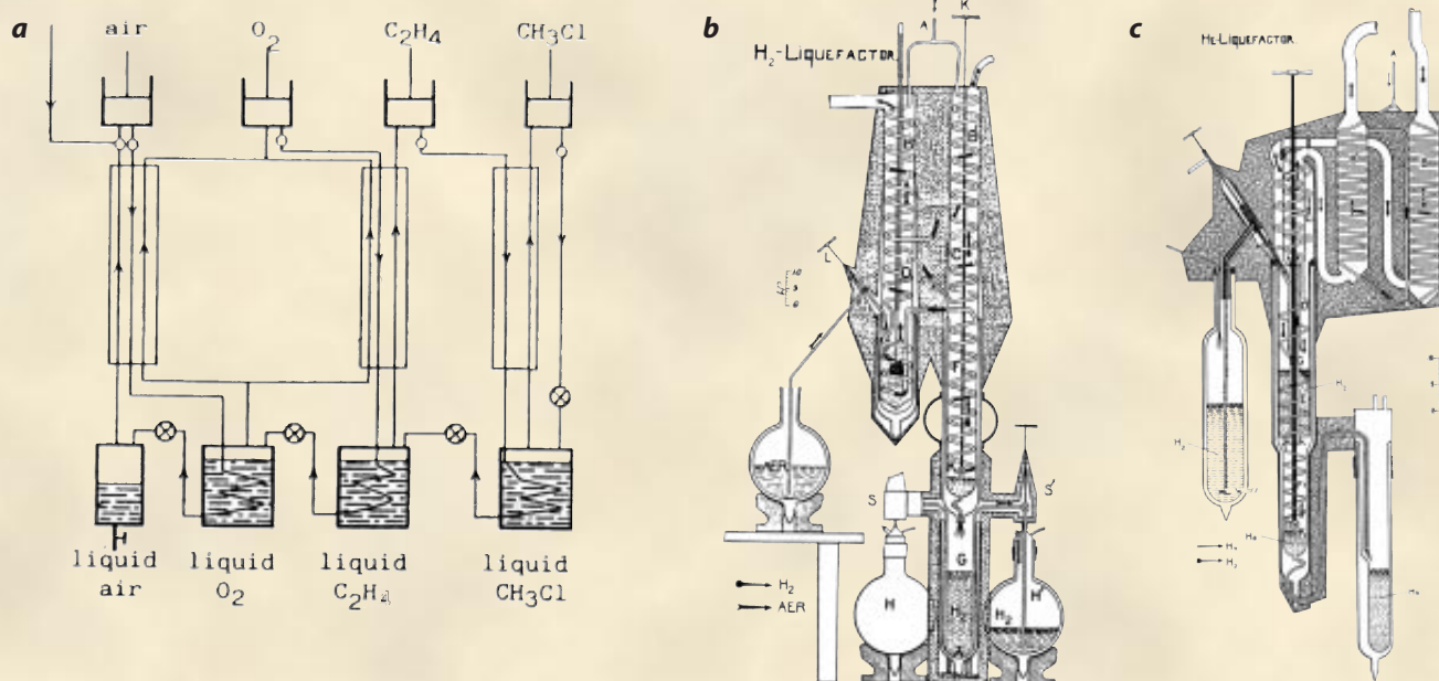
CASCADE APPARATUS (a) constructed by Onnes in 1892 could produce 14 liters of liquid air per hour. Liquid air was essential for operating the hydrogen liquefier (b) he perfected in 1906. The hydrogen gas travels through the system to a liquid air bath and ultimately to an expansion valve, which permits hydrogen gas to expand and liquefy. The liquid hydrogen is collected, while gas returns to the compressor. Onnes developed the first helium liquefier (c) in 1908. He posed with his mentor, Johannes Diderik van der Waals, in front of the device in 1911 (d) and, a decade later, with his chief assistant, Gerrit Flim (e).
