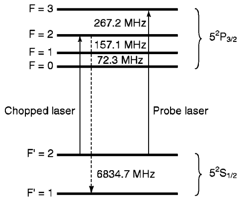
Fig. 2. Partial energy level diagram of \text{Rb}^{87} showing chopped and probe laser transitions. The chopped laser pumps atoms from the F'=2 ground state to the F'=1 state. The probe absorption is sensitive to changes in the F'=2 ground state population.
