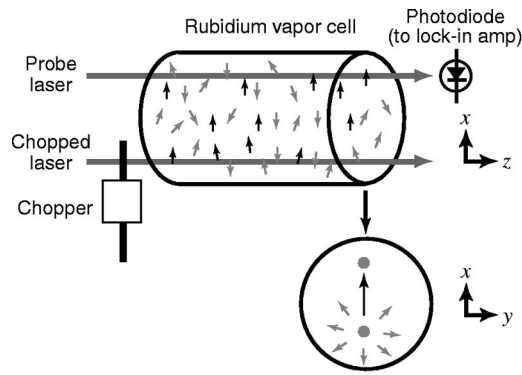
Fig. 1. Experimental arrangement for the observation of a vapor cell atomic beam. Two separated parallel laser beams copropagate through the cell. Atoms travel from one laser (chopped) to the other laser (probe), which detects only those atoms optically pumped by the first laser.
