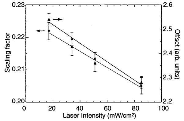
Fig. 6. Scaling and offset between theoretical and experimental results. A straight line fit illustrates the linear effect of optical pumping losses.
