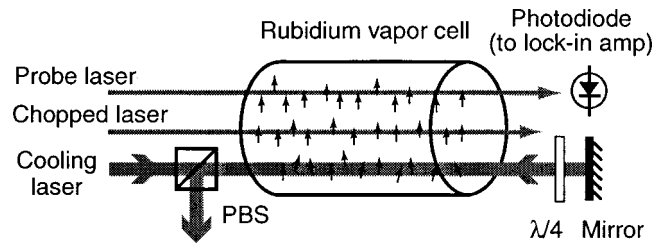
Fig. 4. Experimental arrangement used to observe laser cooling of the vapor cell atomic beam. A third laser was added to cool the atoms before they reached the chopped laser. Atoms that would not normally be part of the vapor cell atomic beam were cooled into the velocity range excited by the chopped laser, increasing the number of atoms in the beam. \lambda/4 represents the quarter-wave retarder and PBS represents the polarizing beamsplitter.
