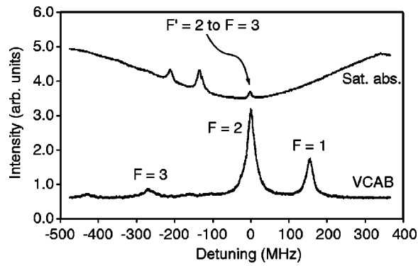
Fig. 3. Lock-in amplifier signal as the probe laser frequency is scanned through the F'=2 to F=3 transition. The top trace is a saturated absorption scan of the probe used to calibrate the probe frequency. The chopped laser was locked to the F'=2 to F=2 transition. VCAB denotes the vapor cell atomic beam signal (probe transmission signal measured through the lock-in).
