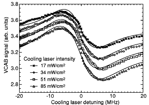
Fig. 5. Measured and predicted lock-in amplifier signals as a function of cooling laser detuning for various cooling laser peak intensities. The symbols are experimental results and the solid lines are theoretical curves.
