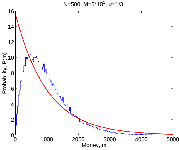
Fig. 4. Histogram: stationary probability distribution of money in the multiplicative random exchange model studied in reference [6]. Solid curve: the Boltzmann-Gibbs law.
