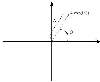
FIG. 3: Ae^{i\theta} has magnitude A and angle \theta . (The “Q” stands for the \theta .) Every time you come across a complex number you should think of this figure. A complex number is a point in a plane with a magnitude (distance from the center) and an argument (angle with the horizontal axis).
