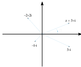
FIG. 1: Complex plane and a few complex numbers
