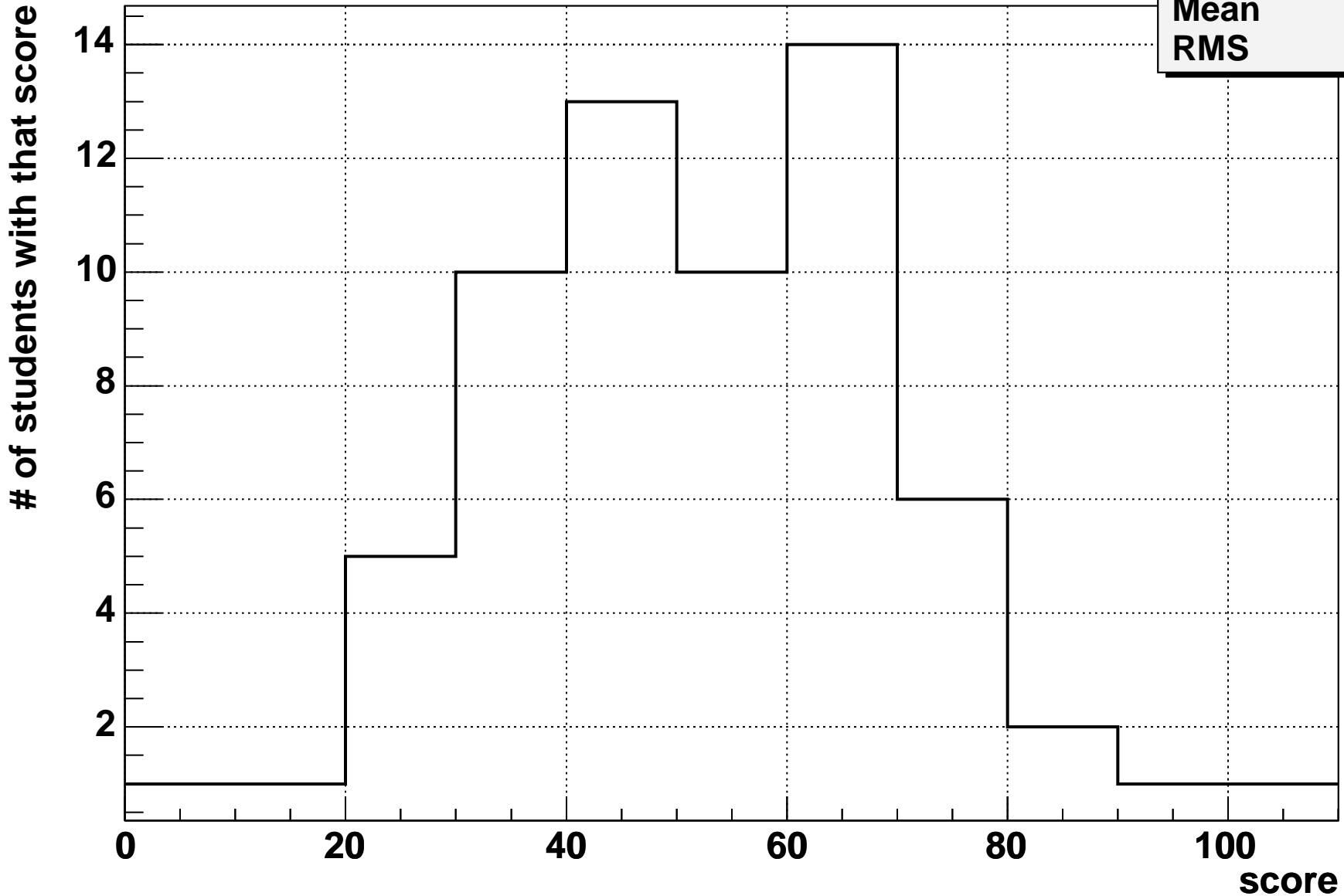
Distribution of scores for Exam 2
