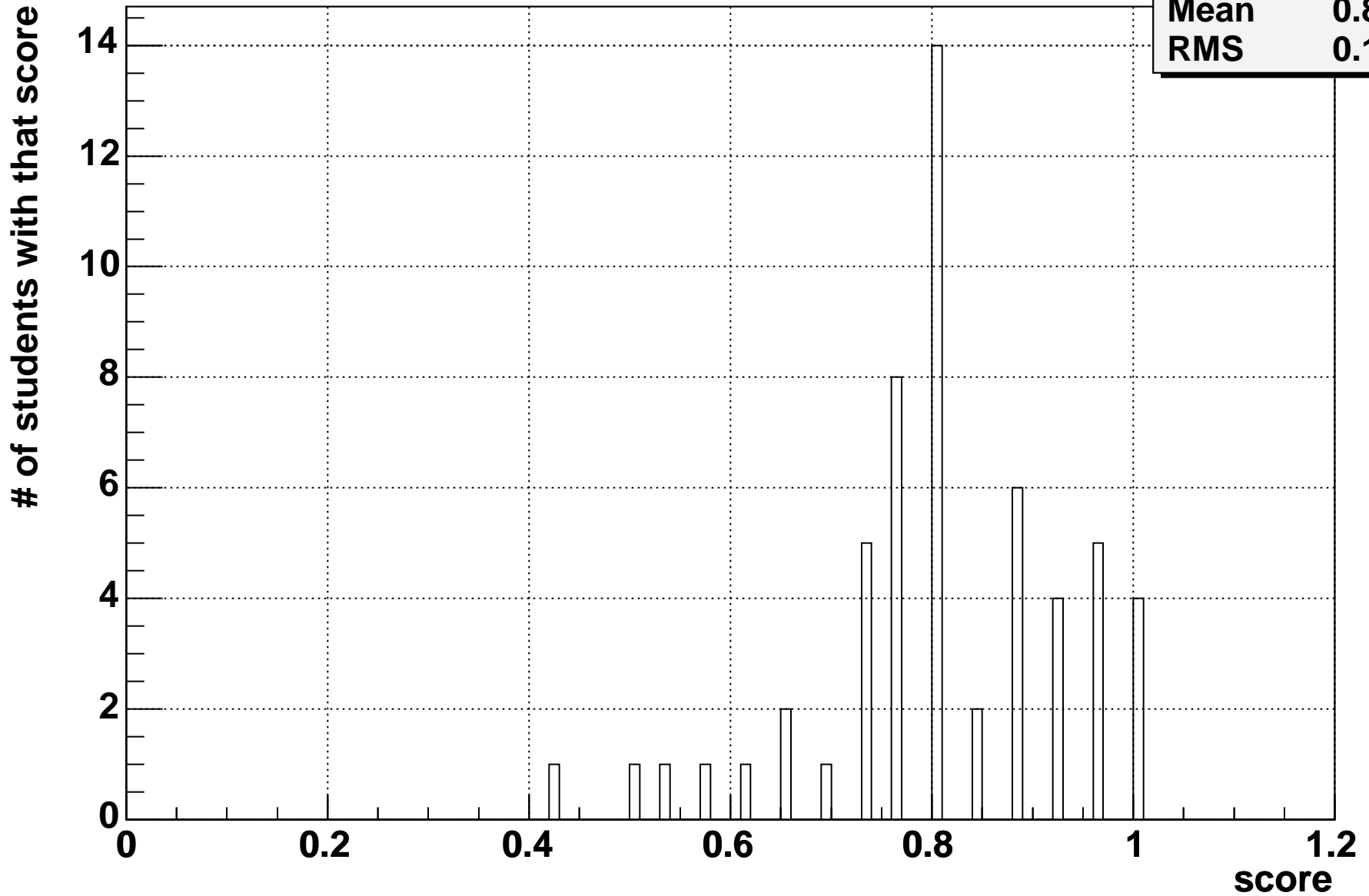
Distribution of scores for HW6
