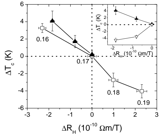
FIG. 5: Change in T_c versus change in R_H at T = 2.5 K. Doping contributions to the change in T_c , \Delta T_c(R_H) , of the x = 0.17 oxygenated samples after the analysis described in the text ( \blacktriangle ). Optimally annealed cerium-doped samples ( \square ). Inset shows the raw data from the oxygenated samples ( \nabla ) along with \Delta T_c(R_H) from the analysis.
