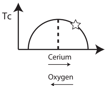
FIG. 1: T_c versus doping phase diagram (schematic) for \text{Pr}_{2-x}\text{Ce}_x\text{CuO}_{4-\delta} . Dashed line indicates optimal cerium doping ( x \simeq 0.15 ). The star on the diagram indicates the Ce doping presented in this paper. Electron carrier concentration increases to the right. Increasing oxygen concentration decreases the electron carrier concentration and is represented by moving to the left. Upon cerium doping, the material becomes more metallic and the residual resistivity decreases as one moves to the right in the diagram.
