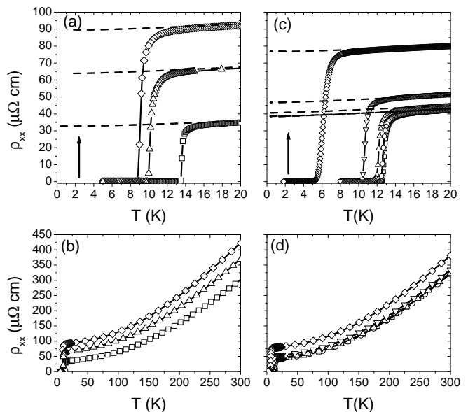
FIG. 2: ab-plane resistivity versus temperature for x = 0.17 cerium-doped PCCO films. Symbols are data taken in zero applied magnetic field. Dashed lines are taken in 10 T field ( H \parallel c -axis) and coincide with H = 0 T above T_c . Scales for (a) and (c) are the same, as well as for (b) and (d). (a) Films with different oxygen content. The arrow indicates the order of increasing oxygen, and the corresponding post-deposition annealing pressures are: 1 \times 10^{-4} ( \square ), 1 \times 10^{-3} ( \triangle ), and 2.3 \times 10^{-1} Torr ( \diamond ). (b) Full temperature scale for the same oxygenated films presented in (a). (c) A single, optimally annealed, film subjected to increasing irradiation doses. The arrow indicates the order of increasing irradiation corresponding to doses 0 ( \square ), 1 ( \circ ), 2.5 ( \triangle ), 8 ( \nabla ), and 32 ( \diamond ) \times 10^{15} ions/cm 2 . (d) Full temperature scale for the irradiated film presented in (c).
