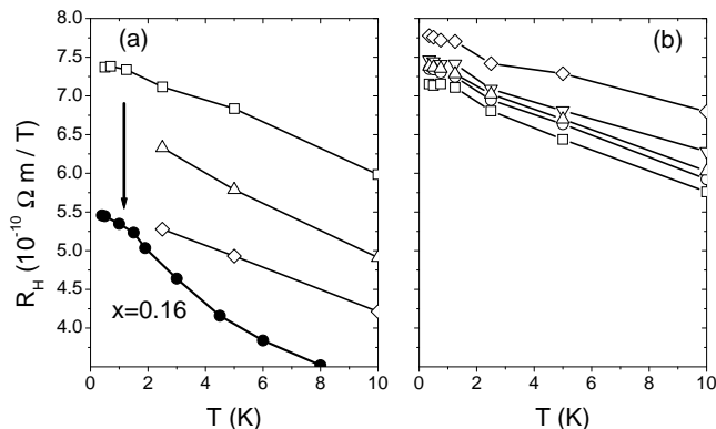
FIG. 3: Hall coefficient ( R_H ) versus temperature for the same films in Fig. 2. Scales for both plots are identical. Although this material is classified as n-doped, R_H is positive on the overdoped side of the doping phase diagram 17 . (a) Films with different oxygen content (arrow indicates order of increasing oxygen). The data labeled x = 0.16 ( \bullet ) is from an optimally annealed x = 0.16 cerium-doped thin film. (b) Single (optimally annealed) film subjected to increasing irradiation doses (arrow indicates order of increasing irradiation dose).
