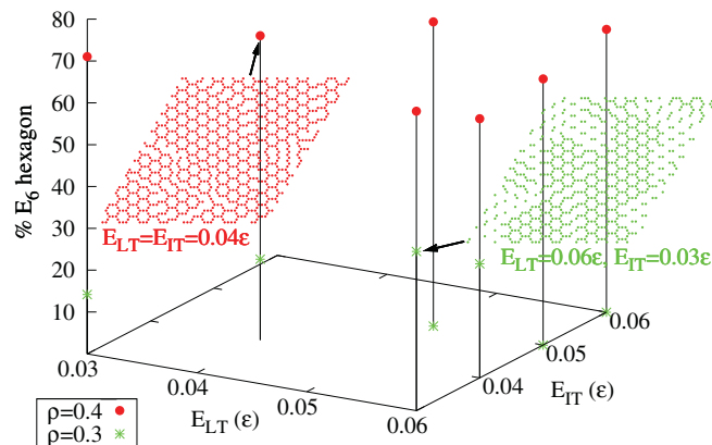
FIG. 12. (Color online) Percentage of E_6 hexagons as a function of the magnitudes of E_{LT} and E_{IT} at \rho = 0.3 (green asterisks) and at \rho = 0.4 (red solid circles). E_T = 0.06\epsilon for both cases. The ground state site configurations are shown at E_{LT} = 0.04\epsilon , E_{IT} = 0.04\epsilon , \rho = 0.4 and at E_{LT} = 0.06\epsilon , E_{IT} = 0.03\epsilon , \rho = 0.3 . For the former and E_{LT} = 0.05\epsilon , E_{IT} = 0.05\epsilon , \rho = 0.4 , there are the same 128 (72.7%) E_6 hexagons, while for the latter there are 67 (38.1%) E_6 hexagons. Obviously, there are more E_6 hexagons for \rho = 0.4 than for \rho = 0.3 .
