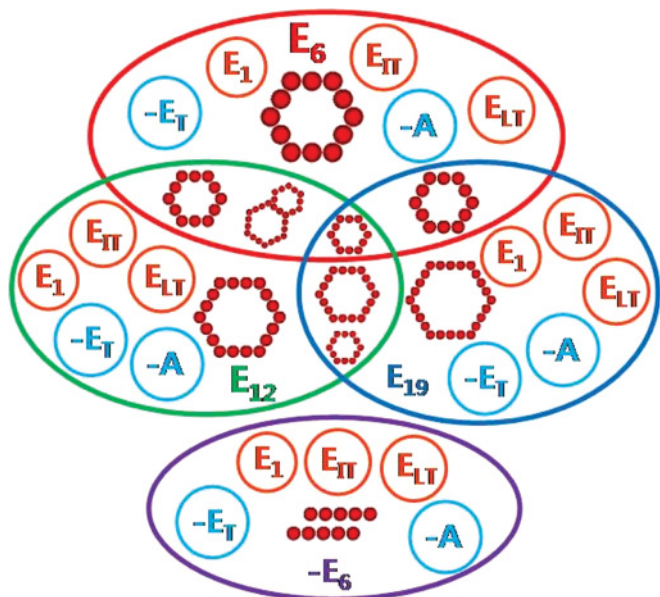
FIG. 14. (Color online) Venn diagram of coupling constants summarizing all of our results. It shows which components are necessary to make which hexagons, also which hexagons form when two or three long-range attractions are present at the same time. For clarity the repulsions are denoted with a negative sign.
