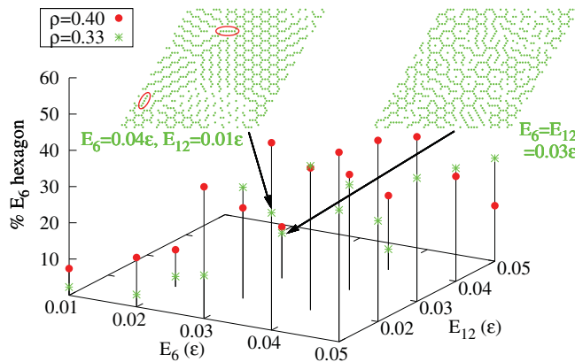
FIG. 10. (Color online) Percentage of E_6 hexagons as a function of the magnitudes of E_6 and E_{12} at \rho = 0.33 (green asterisks) and at \rho = 0.4 (red solid circles). E_T = 0.06\epsilon for both cases. The ground state site configurations are shown at E_6 = 0.04\epsilon, E_{12} = 0.01\epsilon, \rho = 0.33 and at E_6 = 0.03\epsilon, E_{12} = 0.03\epsilon, \rho = 0.33 . For the former there are E_6 hexagons and long straight branches (marked with red ovals) while for the latter both E_6 and E_{12} hexagons are present. Here also there are generally more E_6 hexagons for \rho = 0.4 than for \rho = 0.33 .
