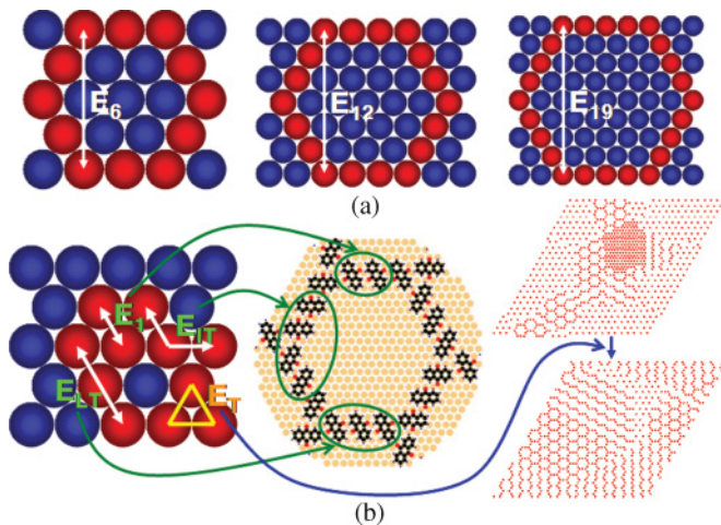
FIG. 1. (Color online) (a) Long-range attractions E_6 , E_{12} , and E_{19} and (b) mappings of the attractive coupling constants ( E_1 , E_{LT} , E_{TR} ) and the trio repulsion constant ( E_T ). Without the trio repulsion, very dense, compact clusters appear, contrary to experiment.
