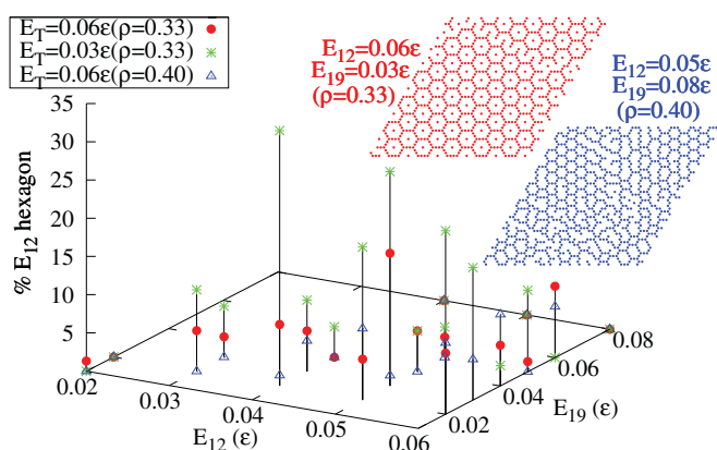
FIG. 5. (Color online) Percentage of E_{12} hexagons as a function of the magnitudes of E_{12} and E_{19} at \rho = 0.33 with E_T = 0.06\epsilon and with E_T = 0.03\epsilon , and at \rho = 0.40 with E_T = 0.06\epsilon . The ground state site configuration is shown at E_{12} = 0.06\epsilon , E_{19} = 0.03\epsilon , \rho = 0.33 with E_T = 0.06\epsilon , of which data point (73 E_{12} hexagons, 97.3%) is not shown in the percentage plot since it is too big compared to the others. The other ground state site configuration is at E_{12} = 0.05\epsilon , E_{19} = 0.08\epsilon , \rho = 0.40 with E_T = 0.06\epsilon , where E_6 hexagons form instead of E_{12} .
