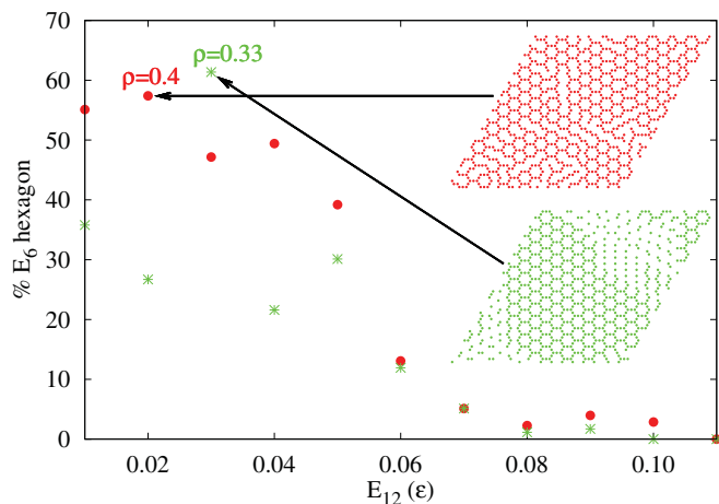
FIG. 9. (Color online) Percentage of E_6 hexagons as a function of the magnitude of E_{12} with a fixed E_6 = 0.06\epsilon at \rho = 0.33 (green asterisks) and at \rho = 0.4 (red solid circles). E_T = 0.06\epsilon for both cases. The ground state site configurations are shown at E_6 = 0.06\epsilon, E_{12} = 0.03\epsilon, \rho = 0.33 and at E_6 = 0.06\epsilon, E_{19} = 0.02\epsilon, \rho = 0.4 , where there are 108 (61.4%) and 101 (57.4%) E_6 hexagons, respectively. Generally there are more E_6 hexagons for \rho = 0.4 than for \rho = 0.33 .
